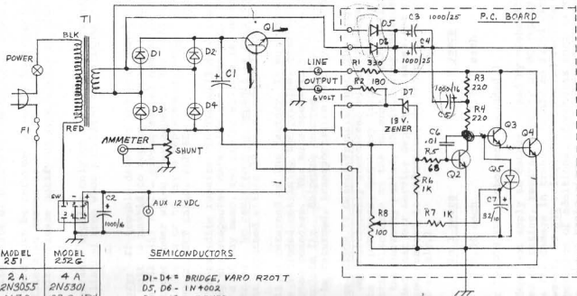
MODELS 251 AND 252G POWER SUPPLIES
